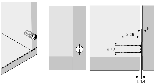
Fitting overlay door, for drill hole installation, lock
