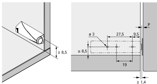
Fitting inset door, for screw on installation, short travel / lock
