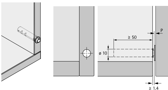
Fitting overlay door, for drill hole installation, short travel
